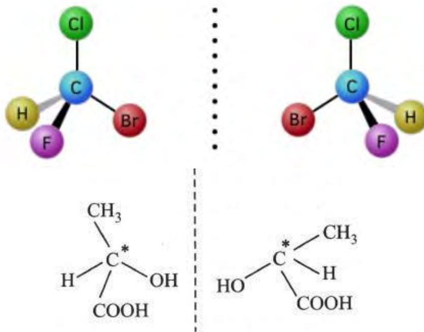
Figure 13.3 Optical isomers
