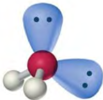
Water, H_2O
